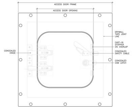
Keyless-Latch
