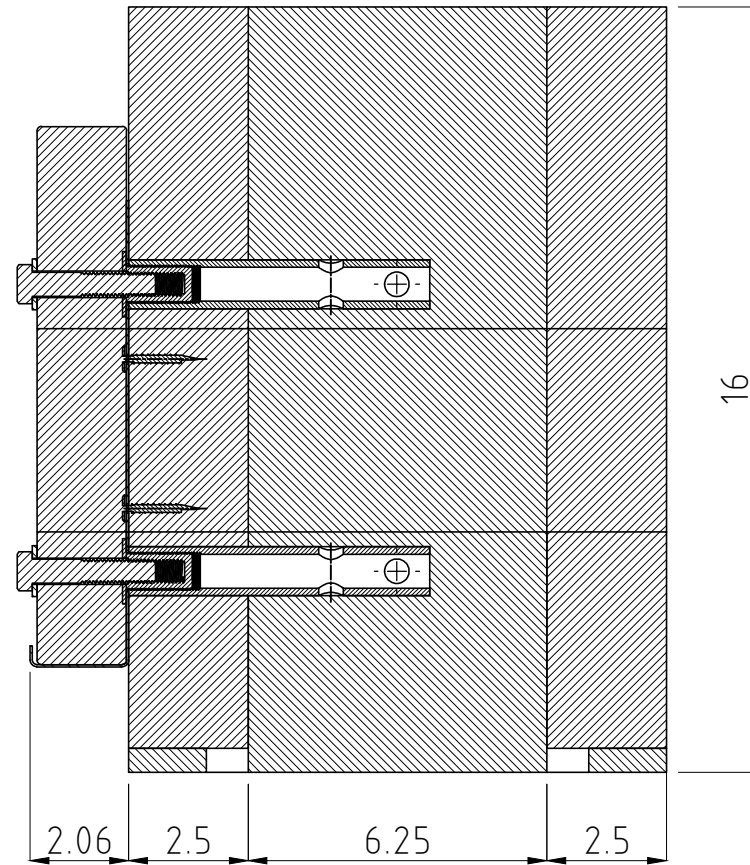
SECTION U-U
