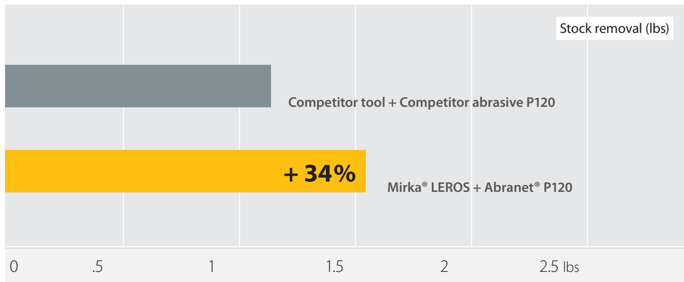
Comparison of stock removal between Mirka LEROS (Abranet P120) and a comparable competitor tool (abrasive grit P120).
